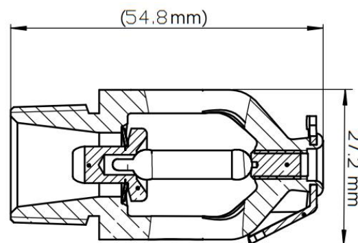
Sidewall Sprinkler Dimension
