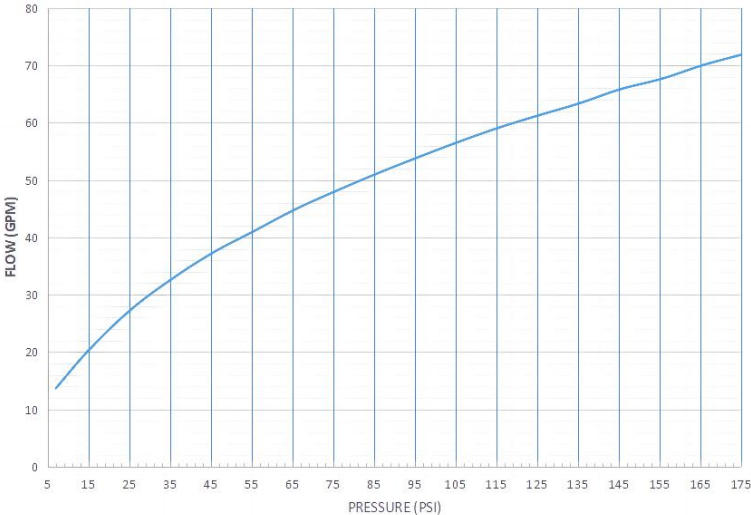
Flow Discharge Chart
