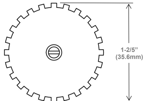
Upright Deflector Dimension
