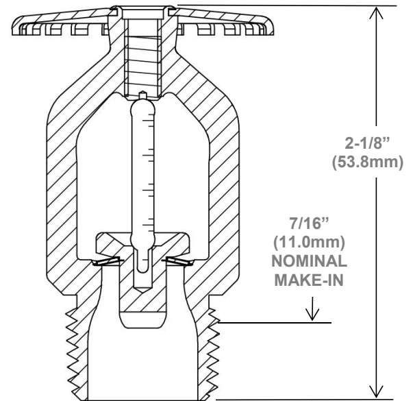
Upright Sprinkler Dimension
